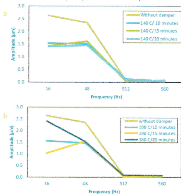
Figure 8. The amplitude value using the frequency domain for: a) Sample S140, b) Sample S180
