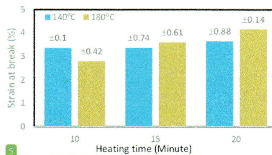
Figure 6. Effect of heating temperature and heating time on strain at break GTR/HDPE
