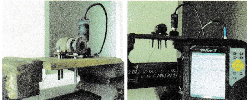
Figure 3. Set up installation for vibration test
