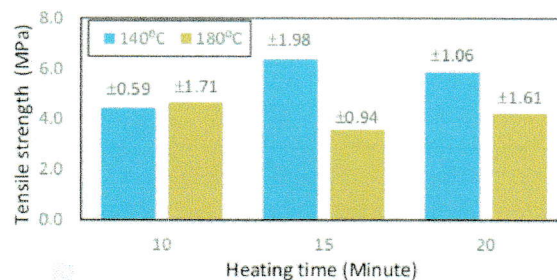
Figure 4. Correlation between heating time and heating temperature to the tensile strength
