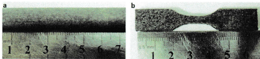
Figure 2. a) HDPE/GTR Blended sample after compaction and heating, b) Tensile test specimen
