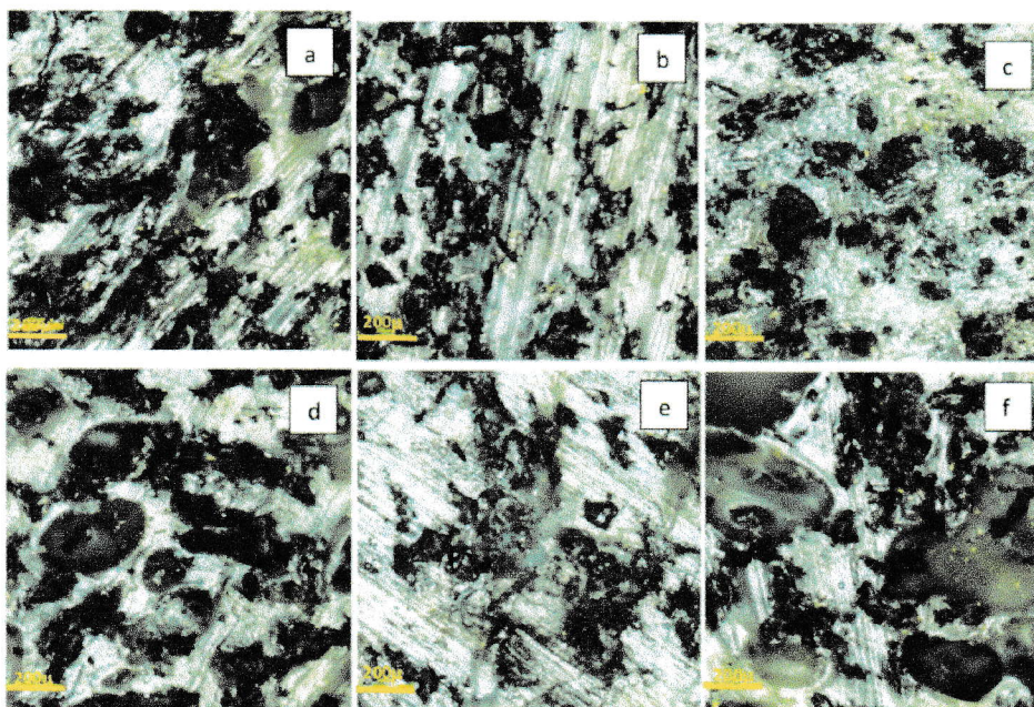
Figure 5. Microstructure of HDPE/GTR blend; a. S140/10; b. S140/15; c. S140/20; d. S180/10; e. 180/15 and f. S180/20
