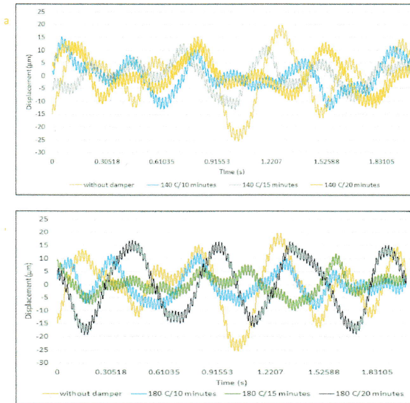
Figure 7. Profile of vibration displacement: a) sample S140, b) sample S180.
